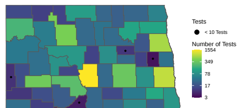
Figure 9: Smoothed number of Radon tests by county.
